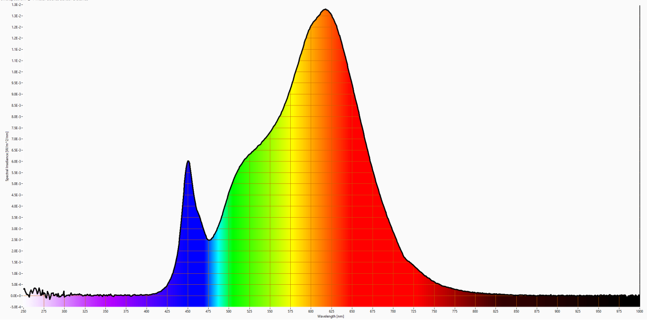
PowerSpectrum @ 1 meter Source Sensor Distance
