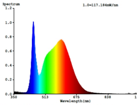
SPL62X62-48W-RGBWWW(at 4000k)
