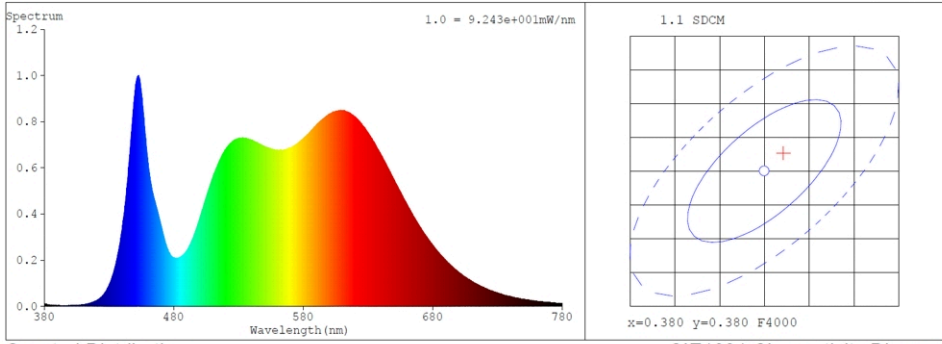
Spectral Distribution
